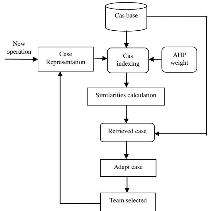
Fig. 2. The structure of a team selection system
